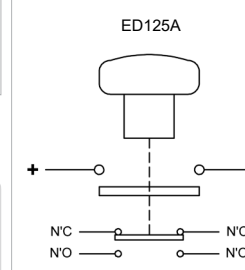
Connection Diagram
