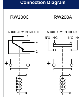
Connection Diagram
